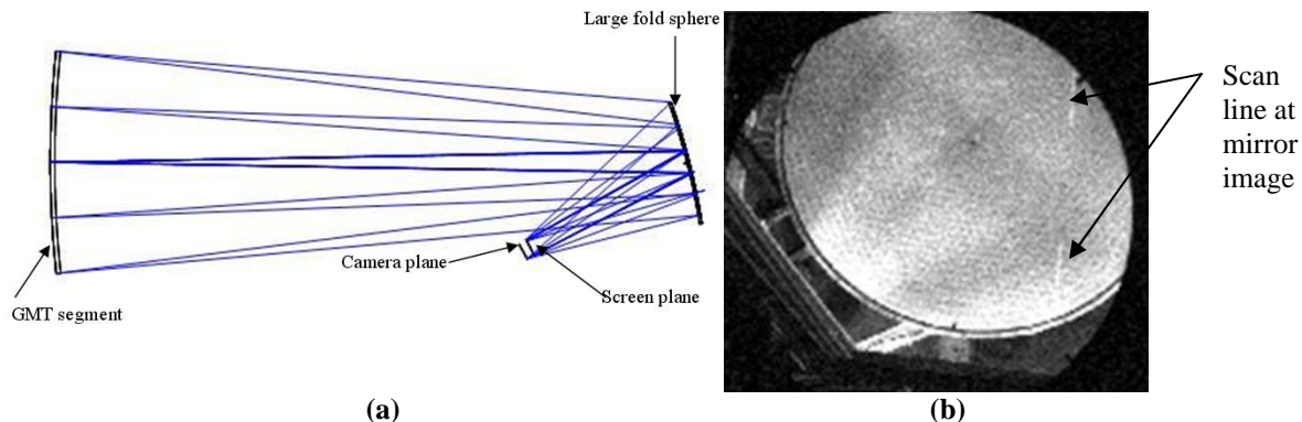
Fig. 4 (a) Basic SCOTS setup for testing the GMT system, (b) initial data where the mirror image shows the corresponding scan line. The line is partially blocked by some mechanical.
