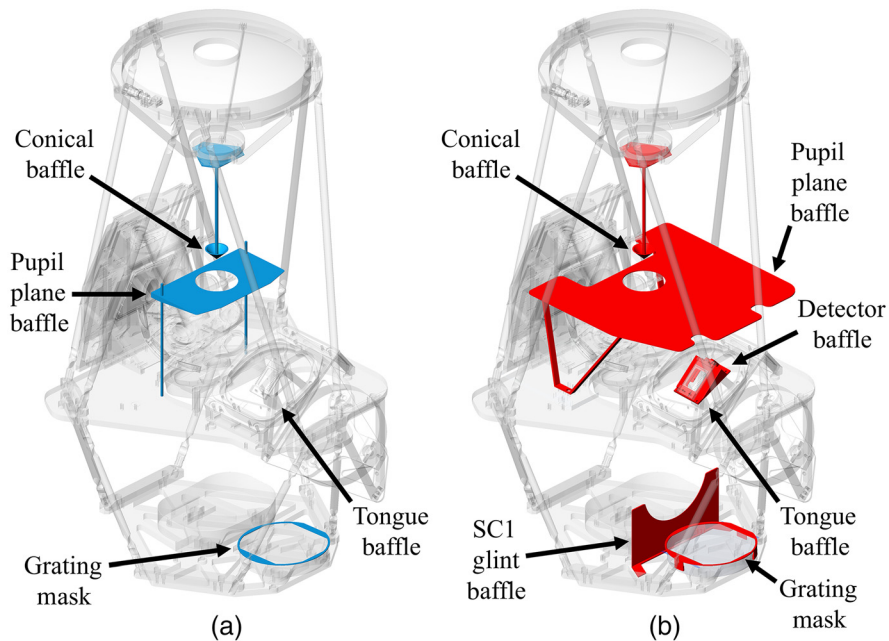
Fig. 5 (a) FIREBall-2 spectrograph configuration from the 2018 flight campaign with baffles highlighted in blue. (b) Updated FIREBall-2 spectrograph with newly added baffles highlighted in red. The conical baffle beneath FC1 was rebuilt, the pupil plane baffle was significantly increased in size, the SC1 glint baffle was added, the grating mask was remade, and the detector baffle was added behind FF2.
