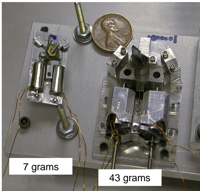
Figure 5. Miniature actuators invented and built at the University of Arizona.
