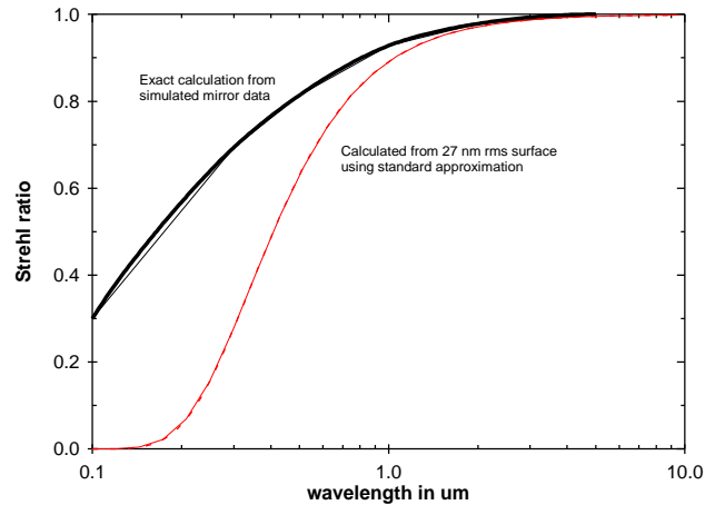
Figure 4. Strehl ratio calculated from simulated figure for the 2-m NMSD.
