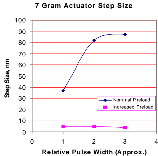
Figure 6. Measured step size for the 7 gram actuator.
