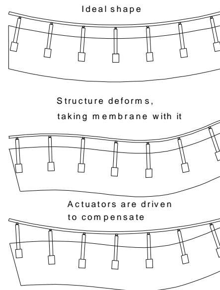
Figure 1. The mirror shape is maintained by making adjustments with actuators, based on wavefront measurements.
