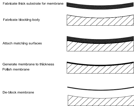
Figure 3. Membrane is carved out of a thicker glass substrate while held to a rigid blocking body with pitch.
