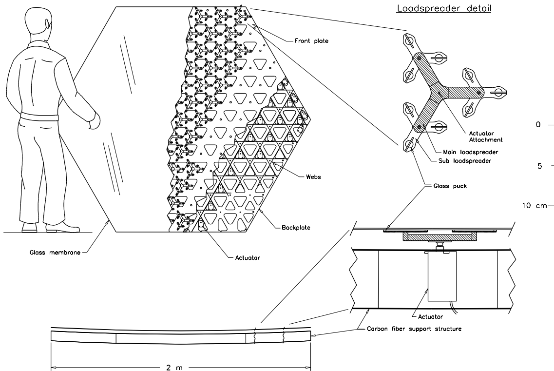
Figure 2. University of Arizona 2-m NGST Mirror System Demonstrator
