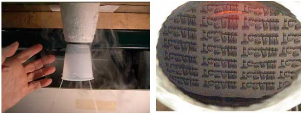
Fig 4. Model of spinning liquid mirror on a superconducting bearing by Ki Bui Ma, University of Houston. (a) shows the bearing, with a nitrogen-cooled YBCO superconductor in the upper cup, and a neodymium magnet in the inverted cup below. The gap is ~ 3 mm. Hanging on 3 strings below is a 20 cm spinning dish of black soy sauce with ~ 8" focal length (b). The lettering is the reflection of a screen above
