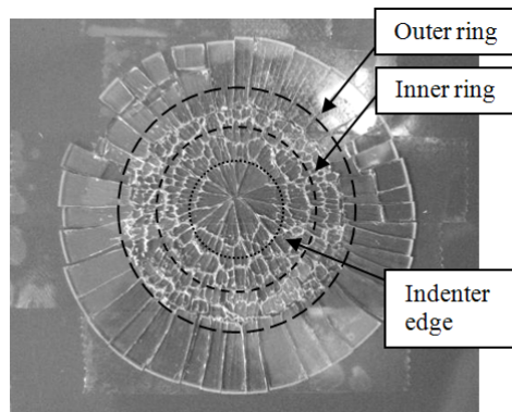
Figure 8. A crack pattern of a sample from a double-ring-test. The dotted rings represent the relative radii among different contact rings on the glass.
