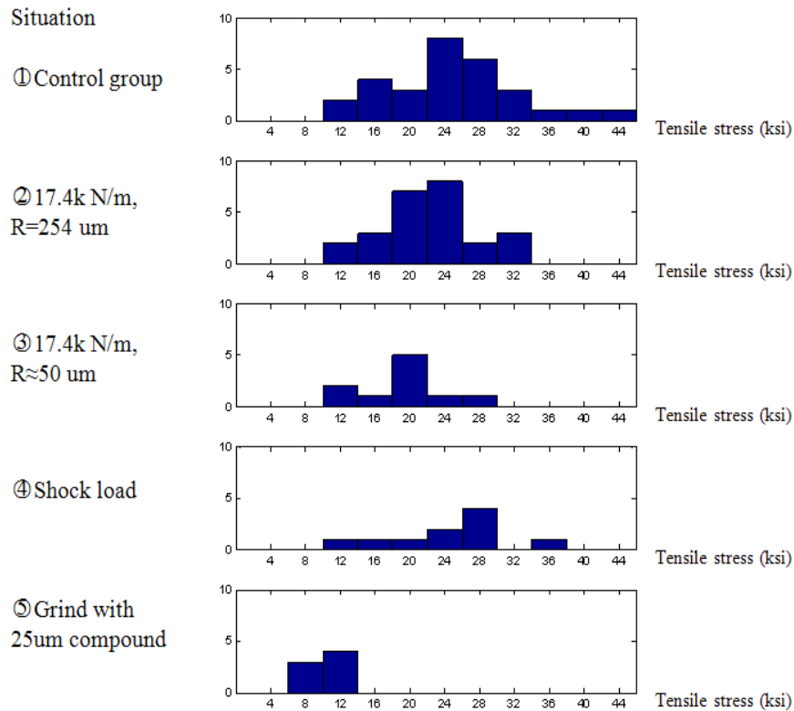
Figure 10. Histograms of the tensile stress values in each situation
