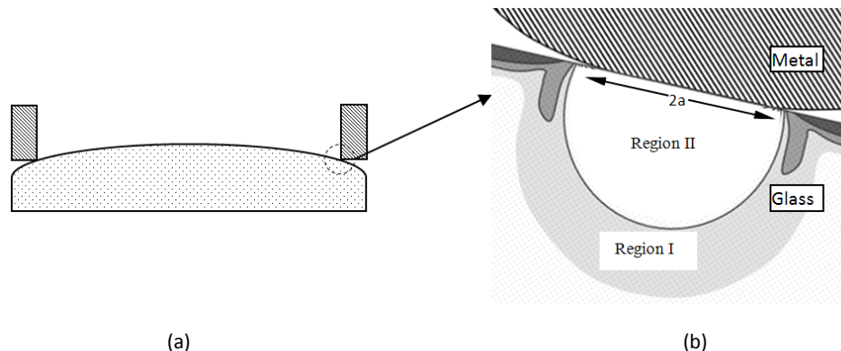
Figure 1. (a) Retaining ring mount, (b) Principle normal stress field 3 . Region I is in tension, while region II is in compression. The maximum tensile stress locates just outside the contact area on the glass surface.
