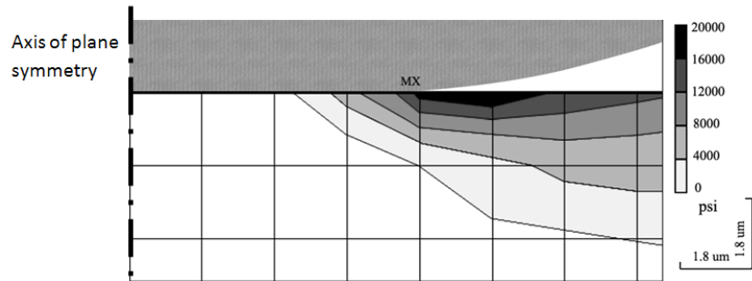
Figure 2. Half-plane tensile stress field on the glass cross section using FEA in ANSYS® frictionless contact.
