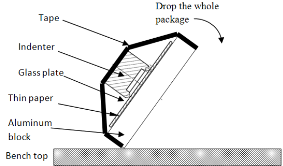
Figure 5. Shock load
