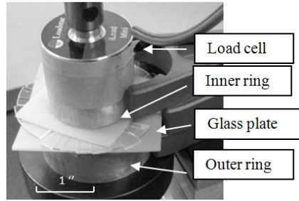
Figure 7. Double ring strength test. Using the same load cell in a different set up, we tested the samples to failure in order to get the strength of the glass compared to the control group.
