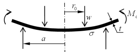
Figure 6. Plate under uniform annular line load
