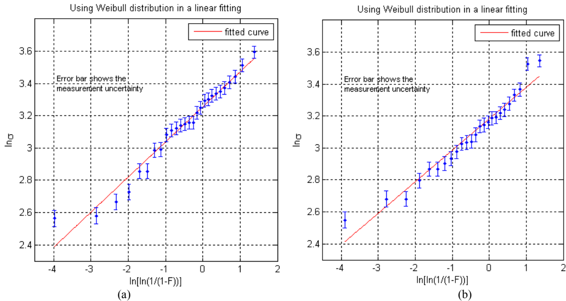
Figure 9. Weibull distribution in a linear fitting. (a) Before exposing to contact stress, (b) After 100 \text{lb}_f/\text{in} loading force. The error bars are the uncertainties in the calculated tensile stresses.
